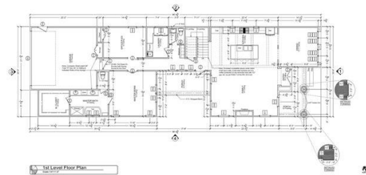
1st Level Floor Plan
